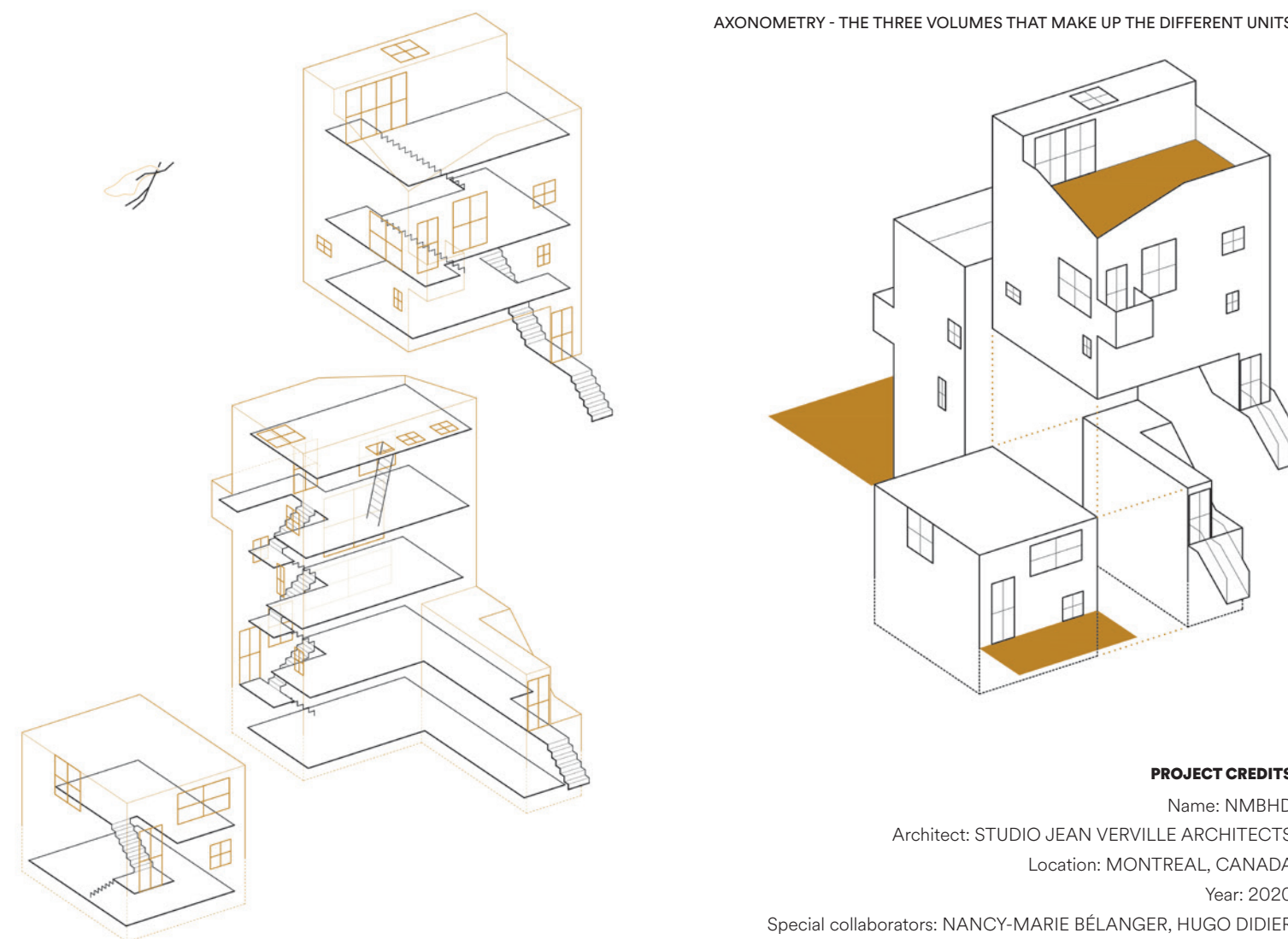
AXONOMETRY - THE THREE VOLUMES THAT MAKE UP THE DIFFERENT UNITS
